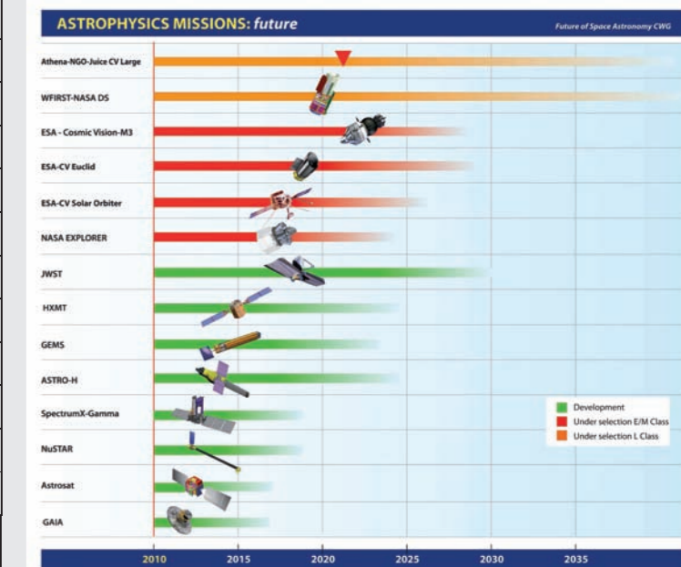
Missions under development (Green), Explorer/Medium class missions under selection processes from ESA and NASA (Red) and the Observatory class mission proposed by the NASA Decadal Survey (DS) and the ESA L-Class mission scheduled for a launch in 2021 (Orange).
